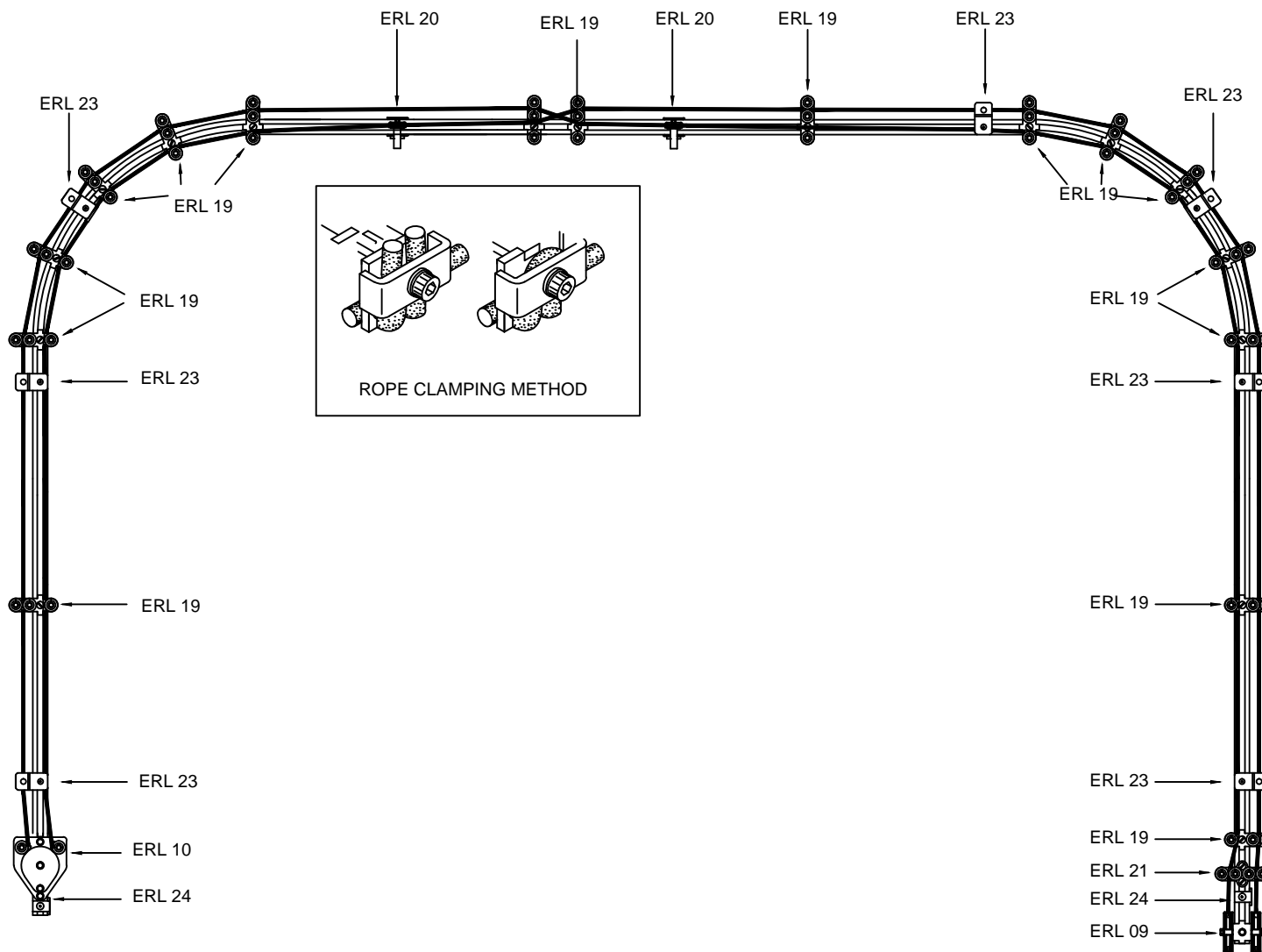
E RAIL CORDING DIAGRAM 06 U-SHAPED OVERLAP ARMS AND CENTRE CROSS OVER VIEWED FROM ABOVE
