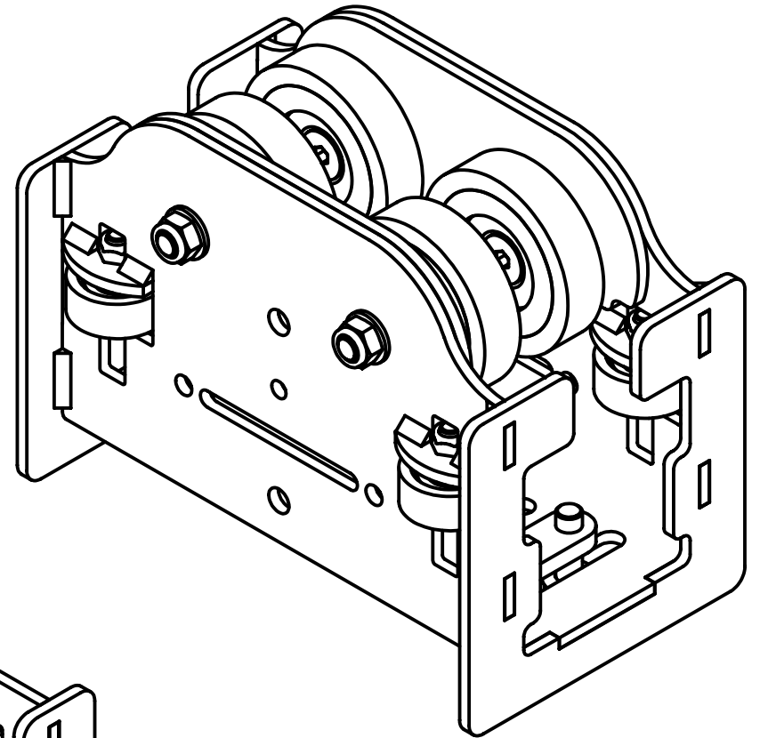
UBM28A Scenery Carrier Top SWL 385kg (Unibeam only)
