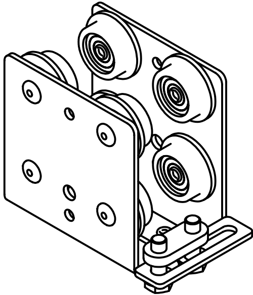
TRA28A Scenery Carrier Top SWL 50kg (Unitrack and Unibeam)
